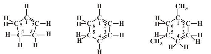
cyclopentene
